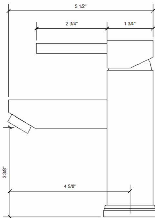
2 Side View 2
